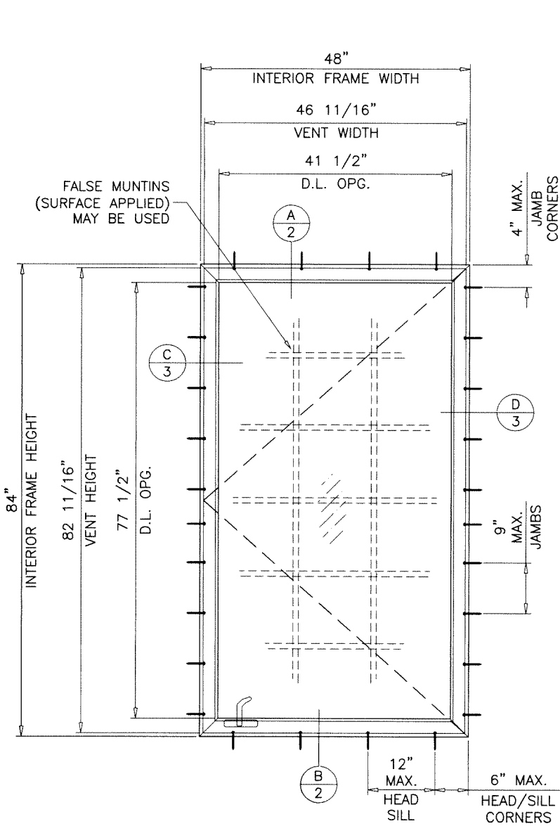
TYPICAL ELEVATION
