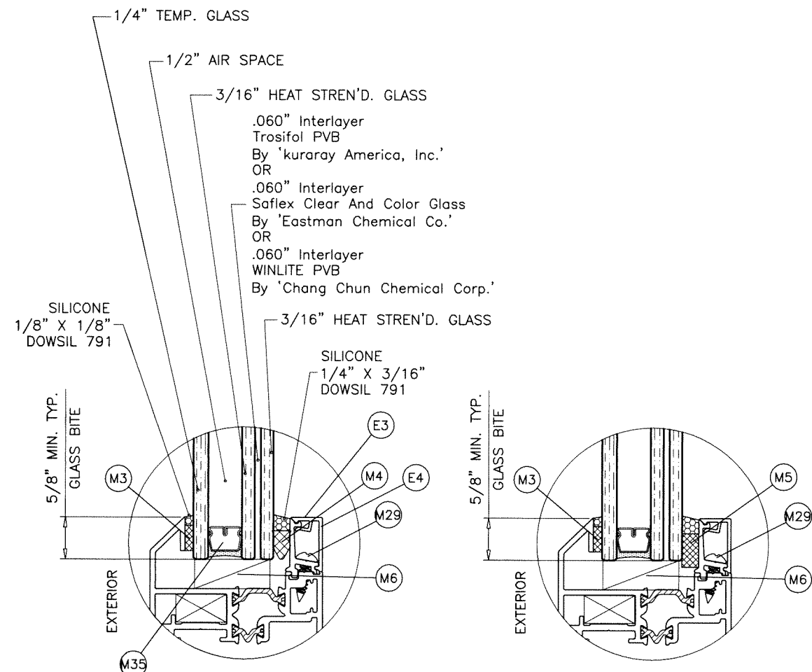
GLASS TYPE 'B' 1-3/16" OVERALL NOM. THK.
