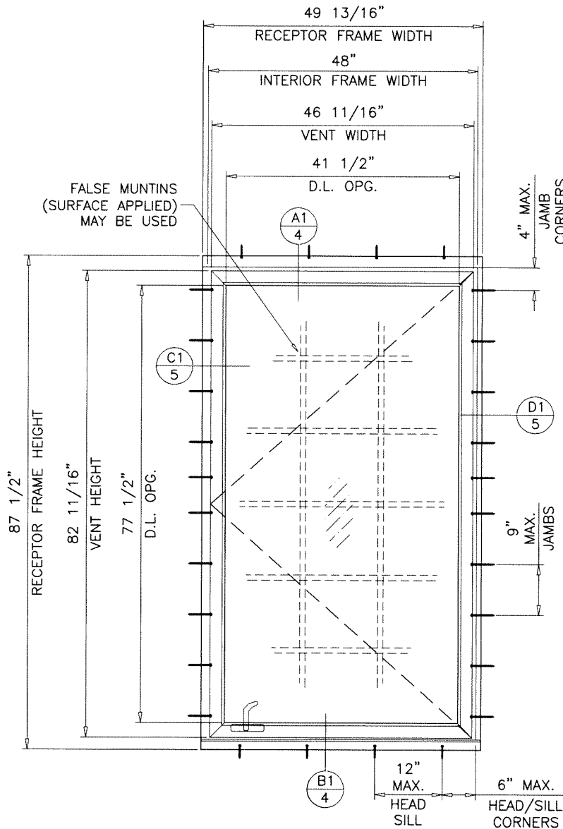
TYPICAL ELEVATION
